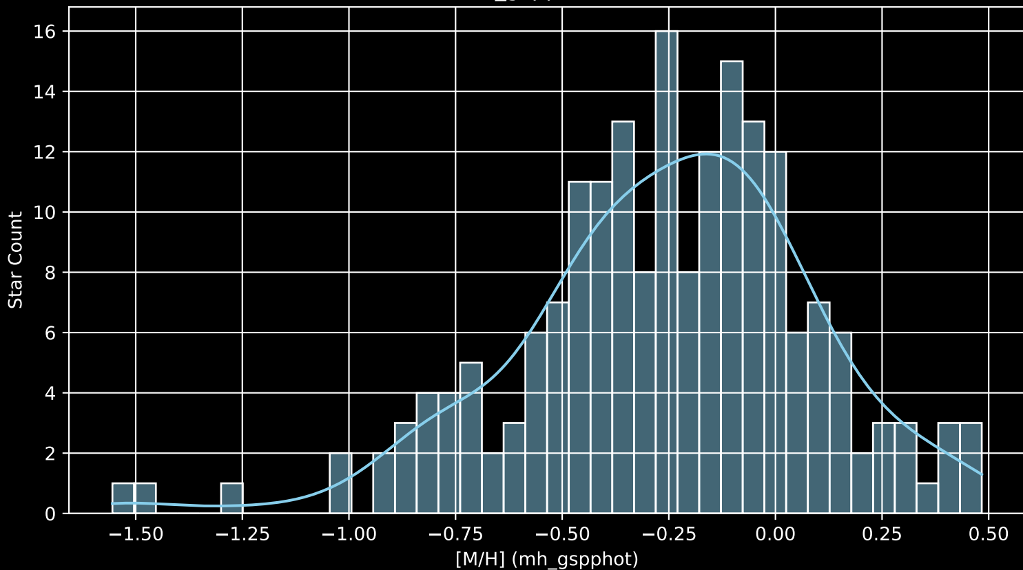
APOGEE DR17 Field: [111+70_MGA [M/H] (mh_gspphot) (n= 194)
