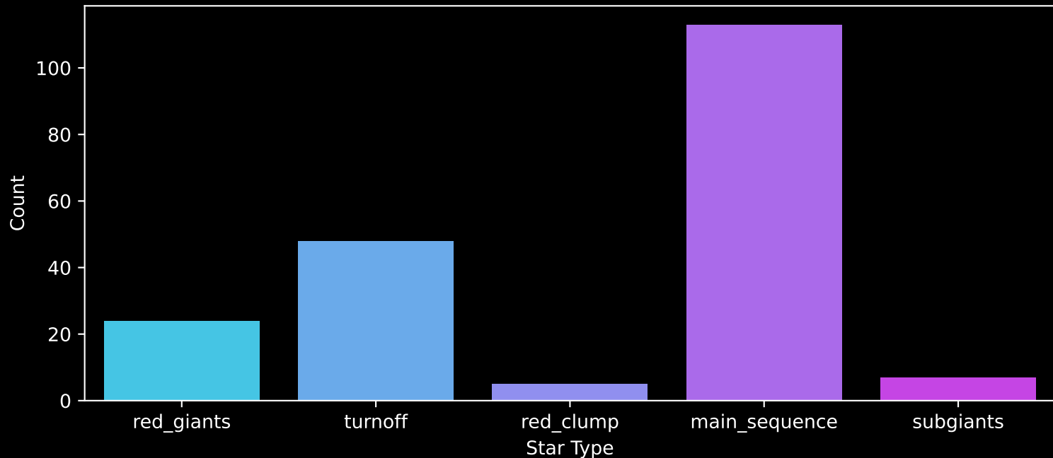
APOGEE DR17 Field: [111+70_MGA] Count plot of Star Type
