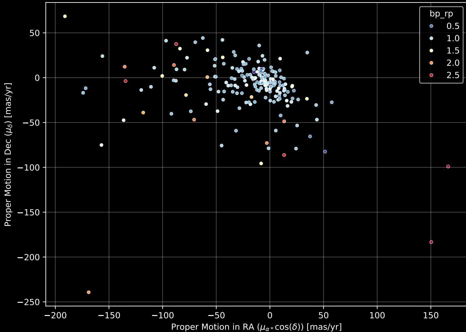
APOGEE DR17 Field: [111+70_MGA] Proper Motion Diagram (n= 197)
