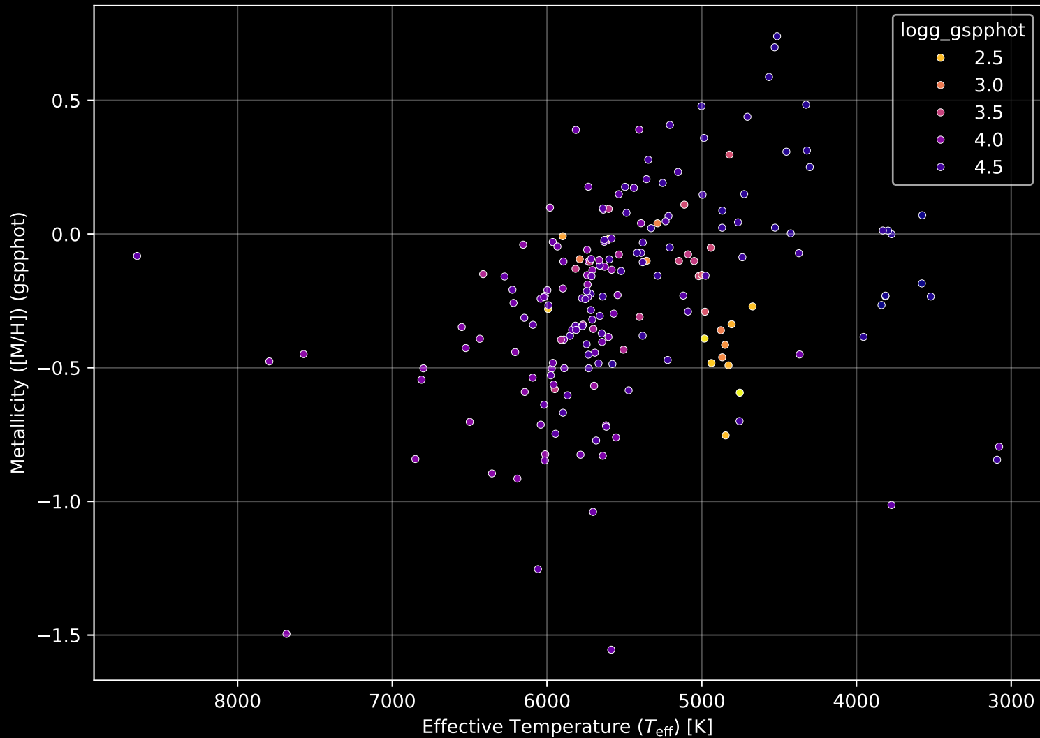
APOGEE DR17 Field: [111+70_MGA] Stellar Population Parameters (n= 197)
