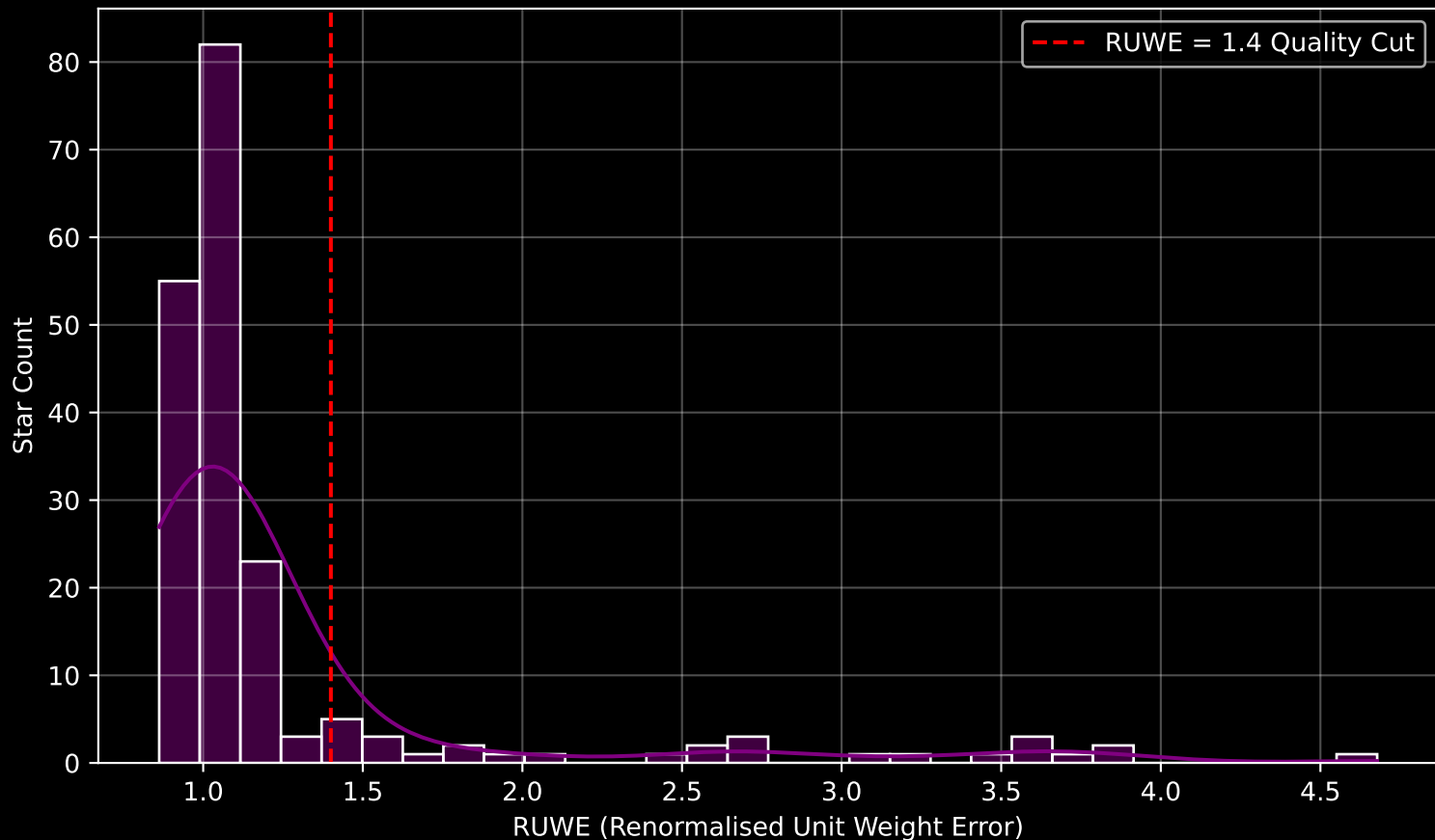
GAPOGEE DR17 Field [111+70_MGA] RUWE Distribution (n= 192)
