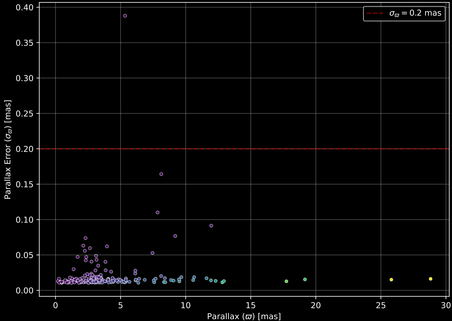
APOGEE DR17 Field: [111+70_MGA] Parallax Quality (n= 197)
